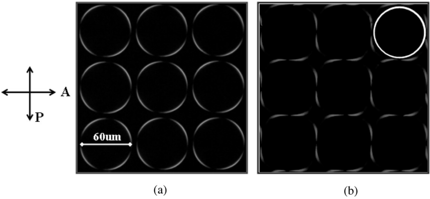
FIGURE 2 Optical microphotographs of (a) LSH-1 cell and (b) LSH-2 cell showing light leakage in a dark state. The circles with white line indicates a hole size of patterned PR.
