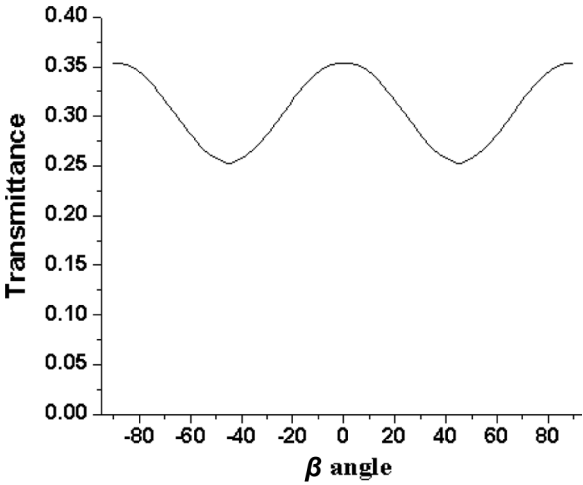
FIGURE 5 Transmittance variation according to angle \beta in the VA-TN.
