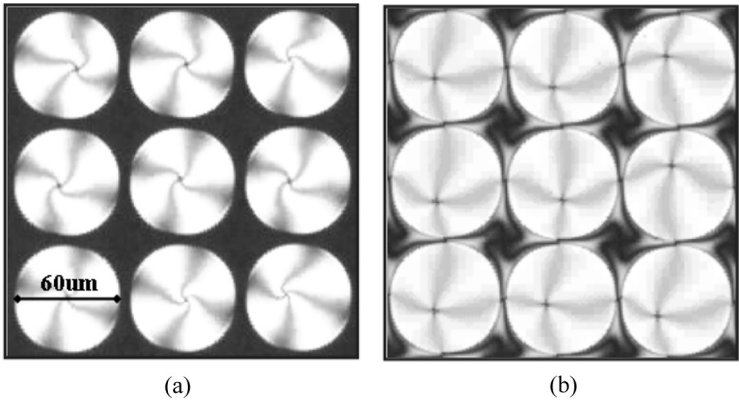
FIGURE 4 Optical microphotographs of (a) LSH-1 cell and (b) LSH-2 cell showing dark brush in a white state at the 5.5 V.
