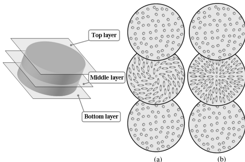
FIGURE 6 The time-resolved textures of LSH-1 cell and LSH-2 cell in crossed polarizers.
