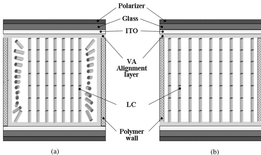
FIGURE 1 Schematic cross-sectional views of (a) LSH-1 cell and (b) LSH-2 cell and the corresponding LC orientation in a dark state.
